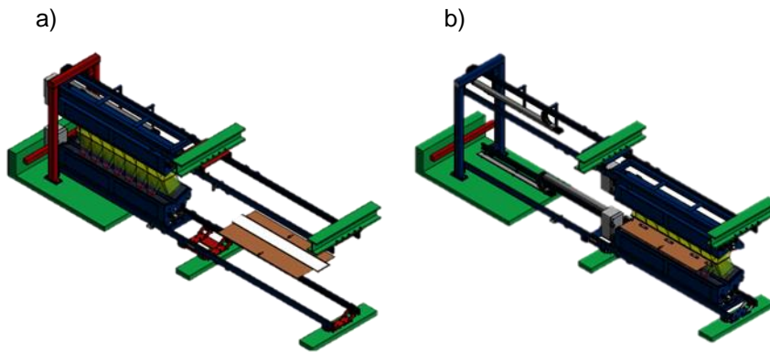
Move Cab system in (a) Maintenance and (b) Inspection position
